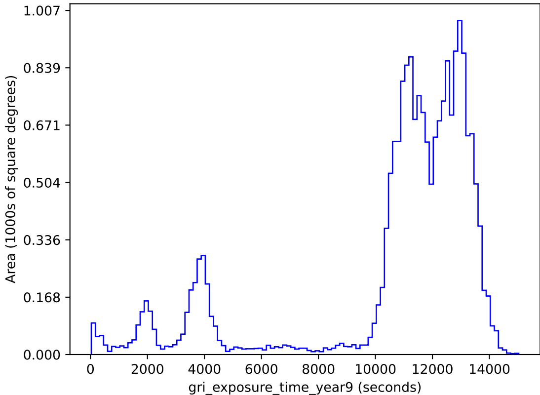
weather_cloudso30v3.4_10yrs gri band non-DD: gri_exposure_time_year9
