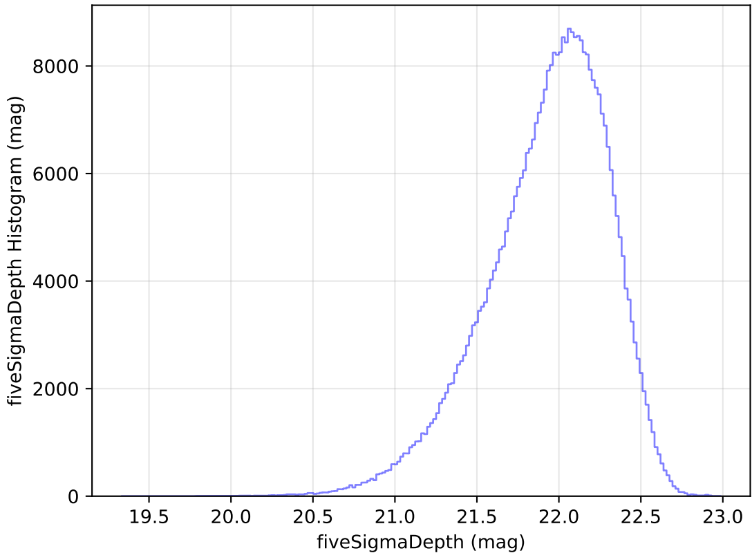
weather_cloudso30v3.4_10yrs y: fiveSigmaDepth Histogram
