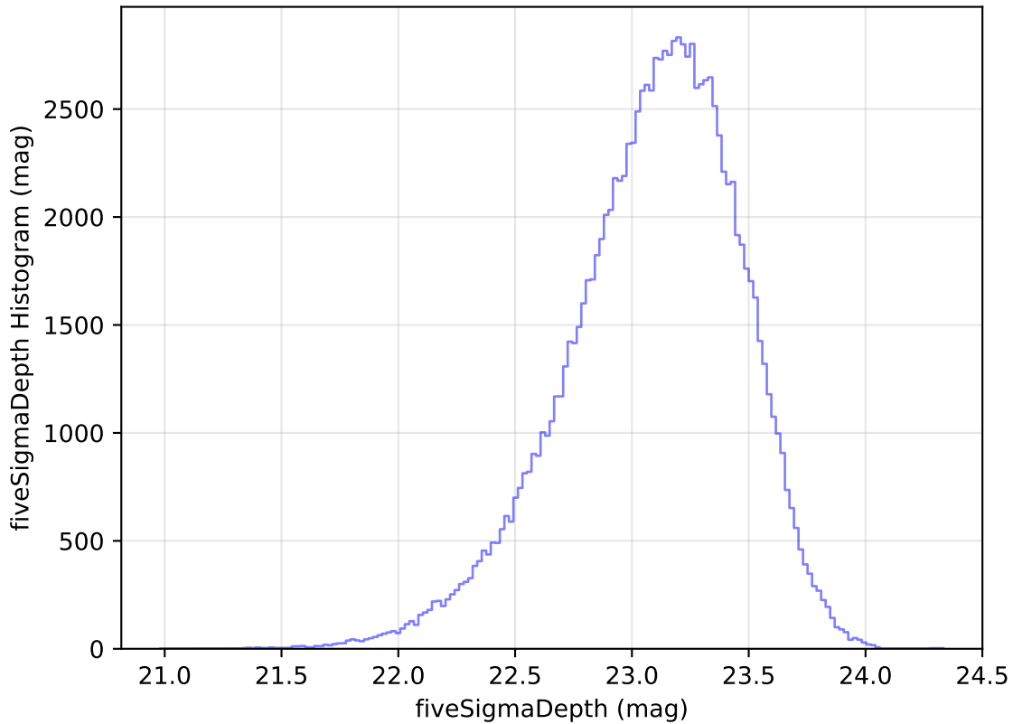
weather_cloudso30v3.4_10yrs u: fiveSigmaDepth Histogram
