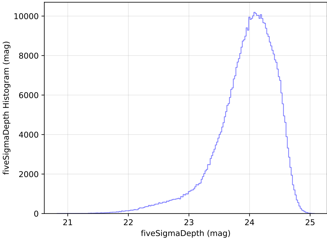
weather_cloudso30v3.4_10yrs r: fiveSigmaDepth Histogram
