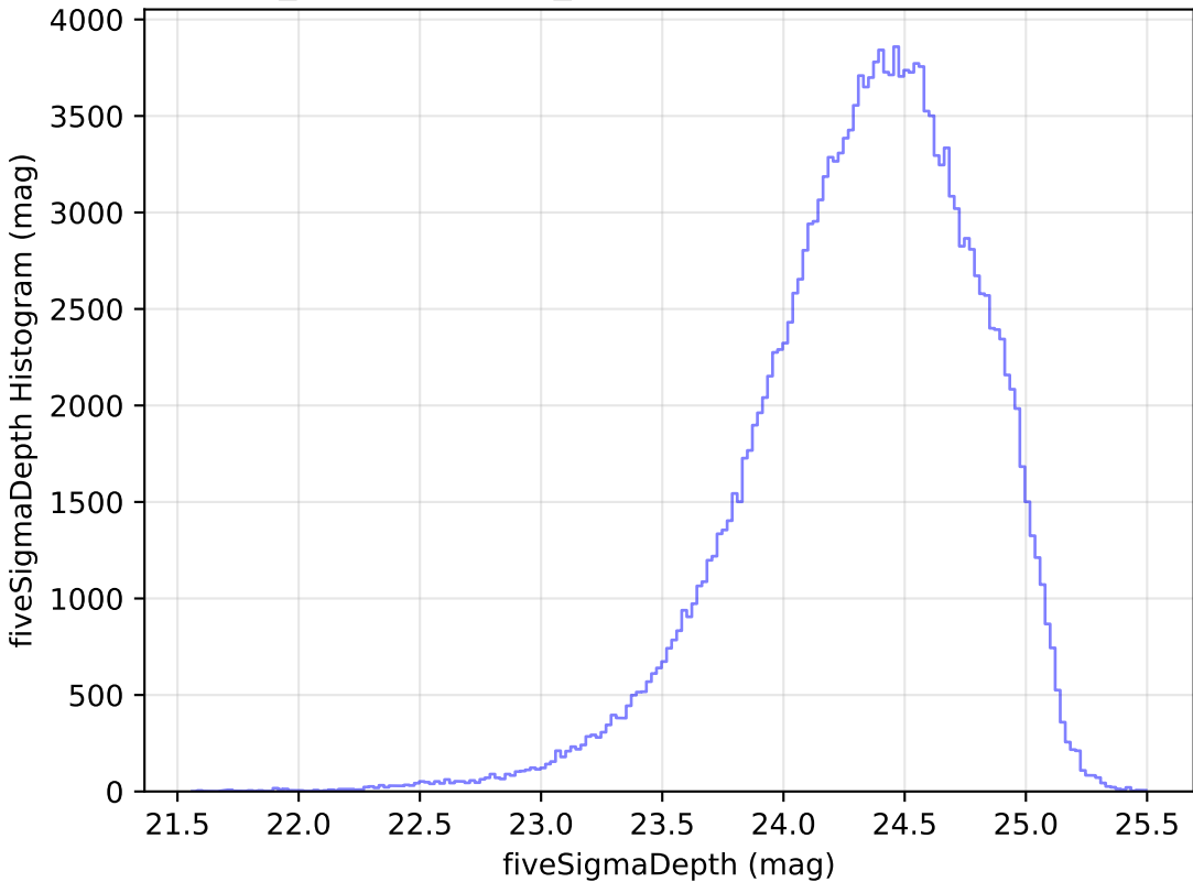
weather_cloudso30v3.4_10yrs g: fiveSigmaDepth Histogram
