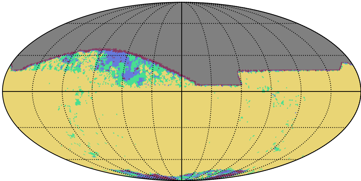
weather_cloudso30v3.4_10yrs z band: YearCoverage night
