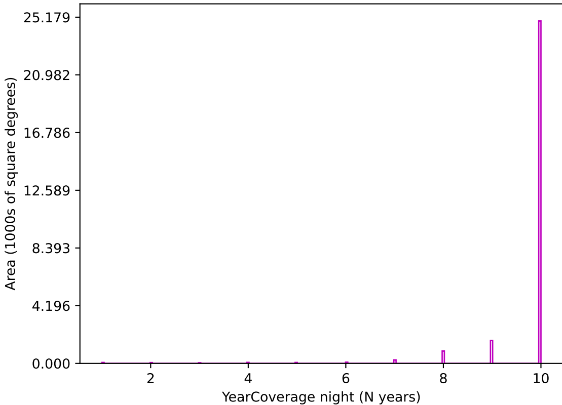
weather_cloudso30v3.4_10yrs z band: YearCoverage night
