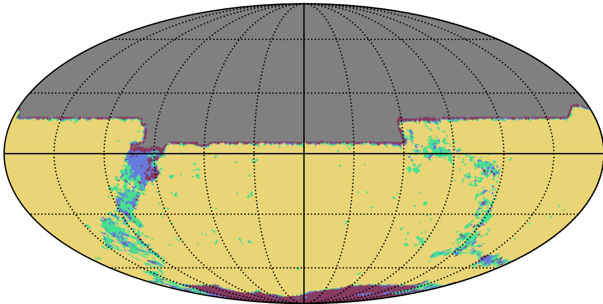
weather_cloudso30v3.4_10yrs y band: YearCoverage night
