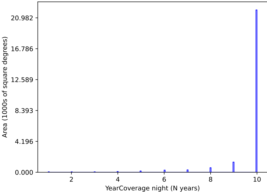
weather_cloudso30v3.4_10yrs y band: YearCoverage night
