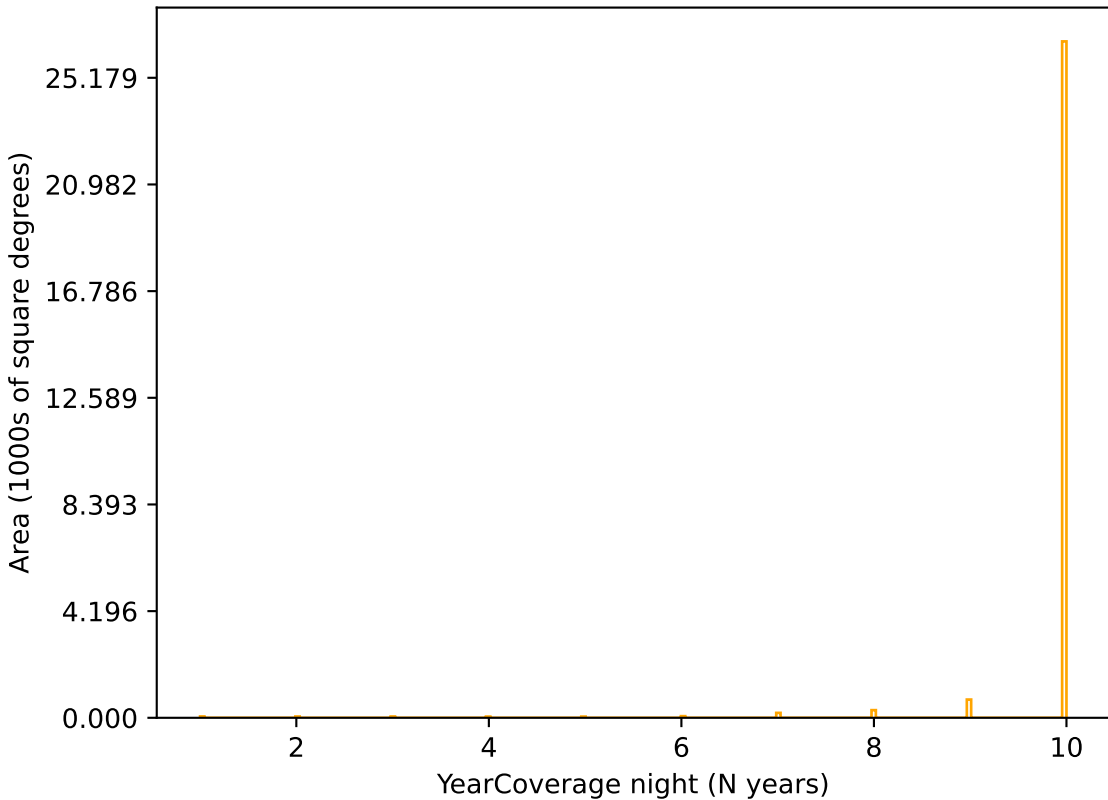
weather_cloudso30v3.4_10yrs r band: YearCoverage night
