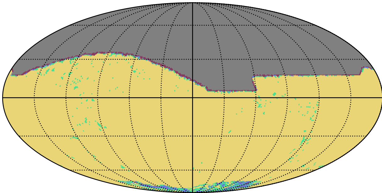
weather_cloudso30v3.4_10yrs i band: YearCoverage night
