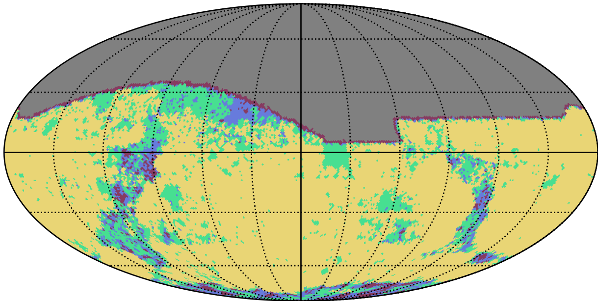
weather_cloudso30v3.4_10yrs g band: YearCoverage night
