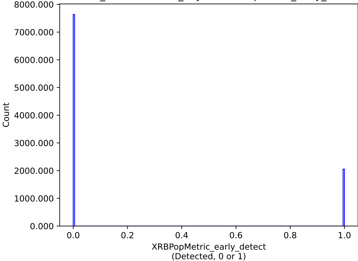
weather_cloudso30v3.4_10yrs : XRBPoMetric_early_detect
