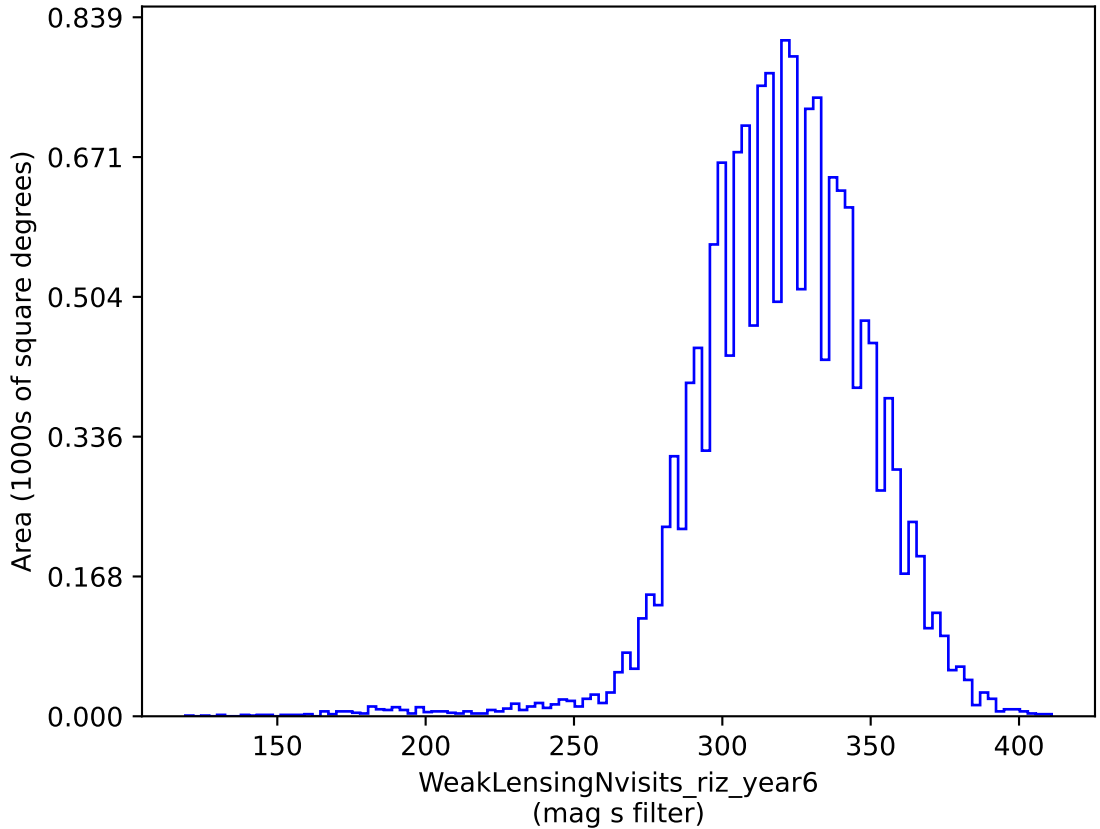
weather_cloudso30v3.4_10yrs gri band non-DD: WeakLensingNvisits_riz_year6
