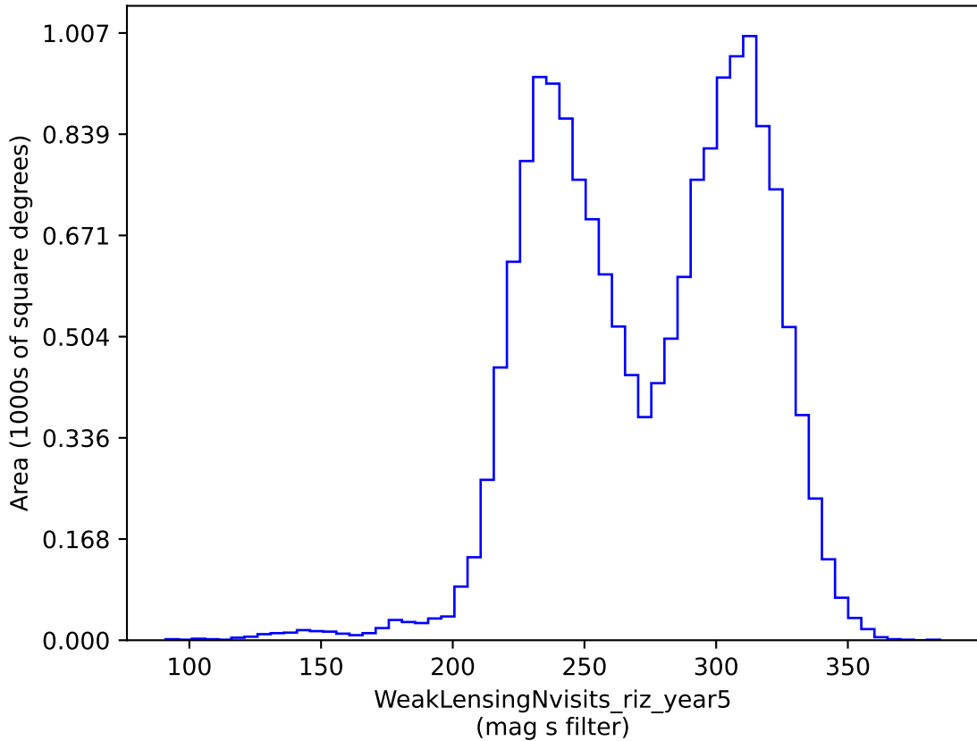
weather_cloudso30v3.4_10yrs gri band non-DD: WeakLensingNvisits_riz_year5
