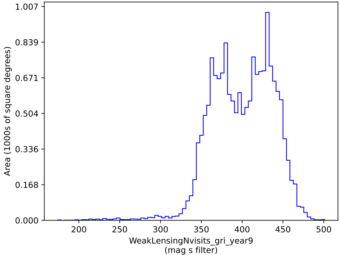
weather_cloudso30v3.4_10yrs gri band non-DD: WeakLensingNvisits_gri_year9
