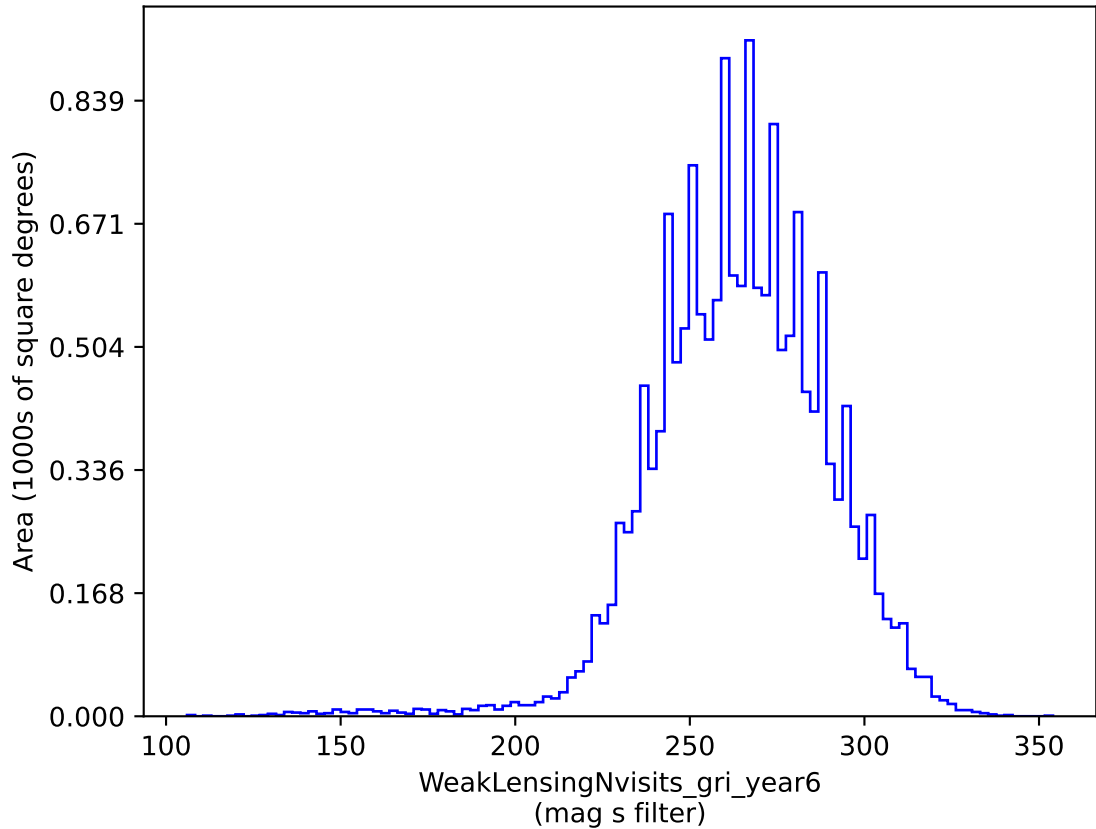
weather_cloudso30v3.4_10yrs gri band non-DD: WeakLensingNvisits_gri_year6
