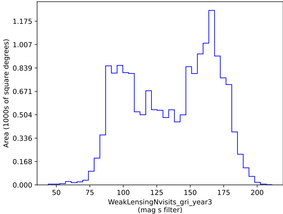
weather_cloudso30v3.4_10yrs gri band non-DD: WeakLensingNvisits_gri_year3
