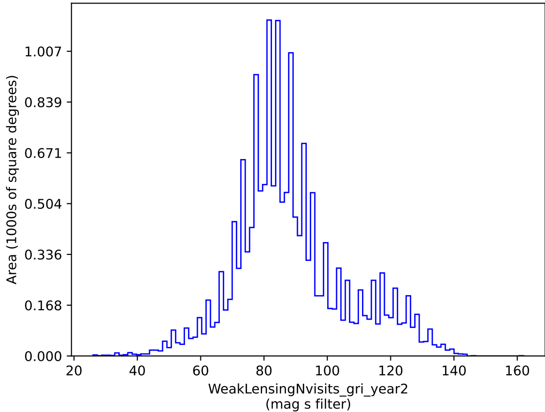
weather_cloudso30v3.4_10yrs gri band non-DD: WeakLensingNvisits_gri_year2
