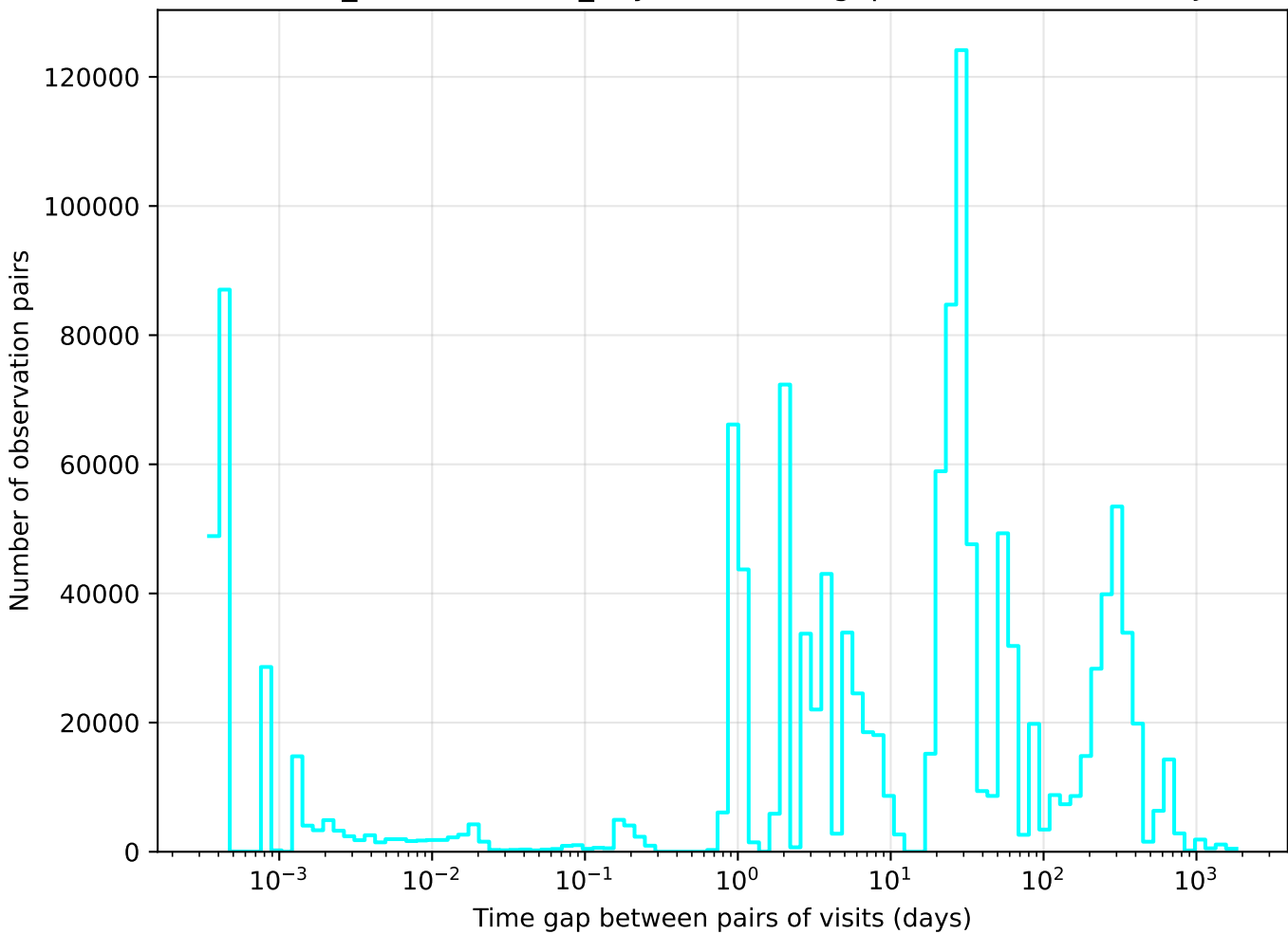
weather_cloudso30v3.4_10yrs u band: Tgaps observationStartMJD
