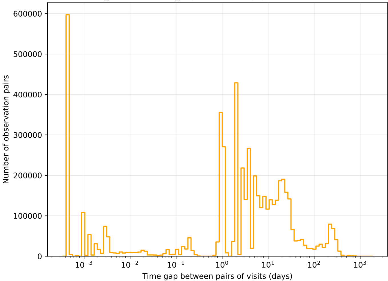
weather_cloudso30v3.4_10yrs r band: Tgaps observationStartMJD
