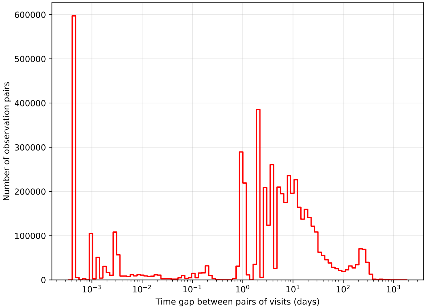
weather_cloudso30v3.4_10yrs i band: Tgaps observationStartMJD
