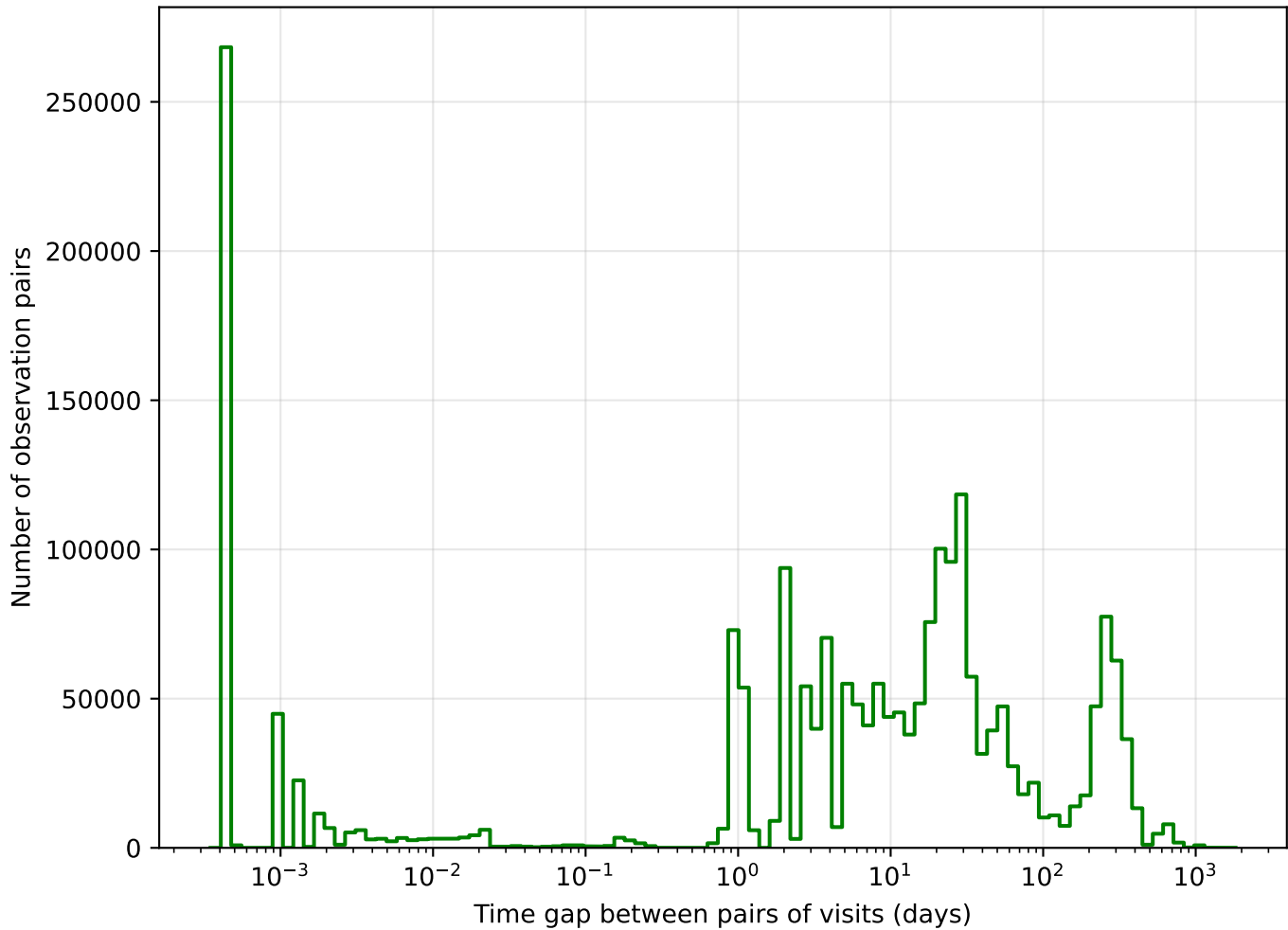
weather_cloudso30v3.4_10yrs g band: Tgaps observationStartMJD
