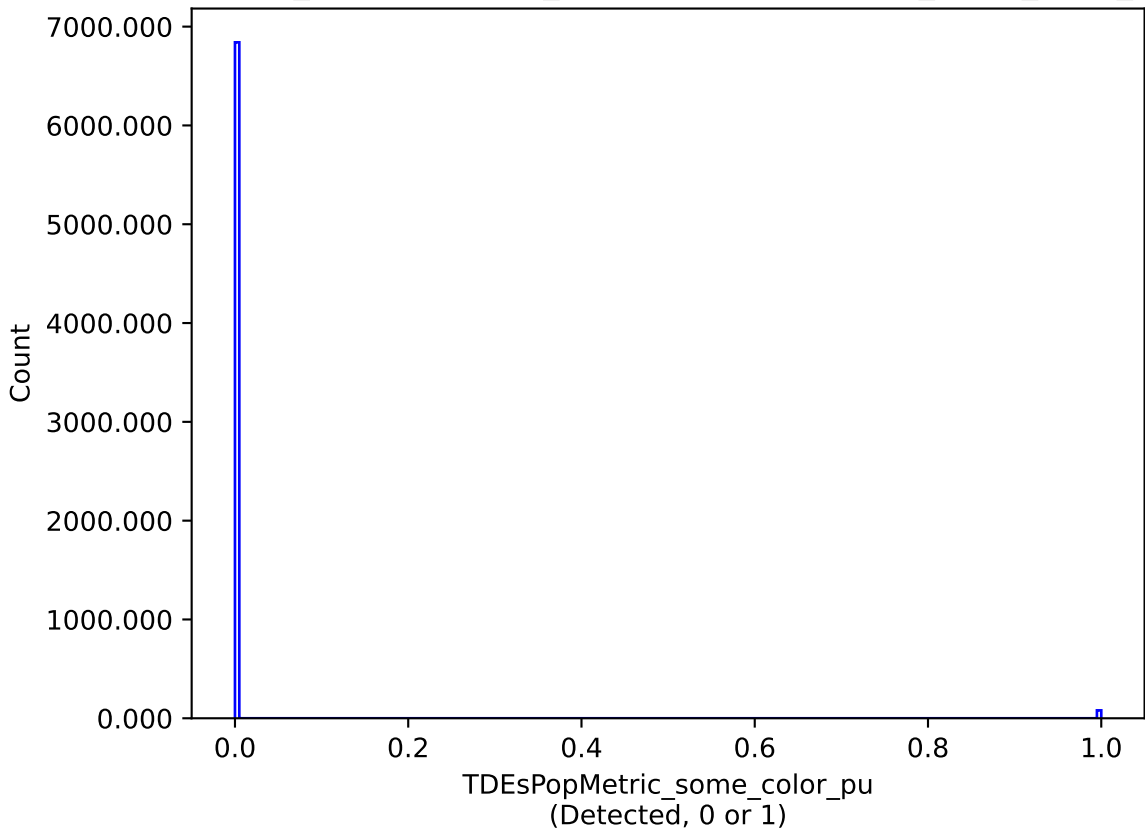
weather_cloudso30v3.4_10yrs : TDEsPopMetric_some_color_pu
