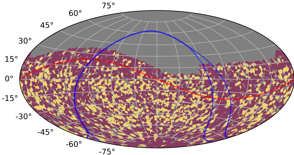
weather_cloudso30v3.4_10yrs : TDEsPopMetric_prepeak
