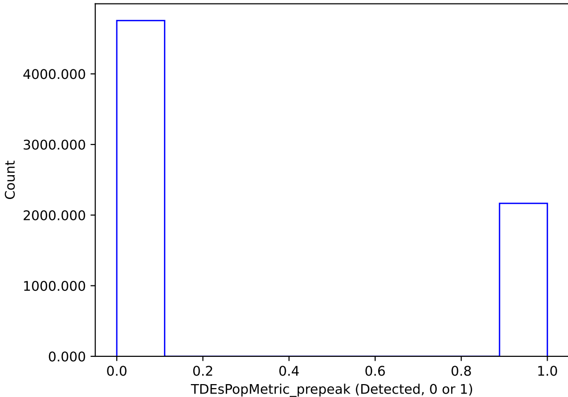
weather_cloudso30v3.4_10yrs : TDEsPopMetric_prepeak
