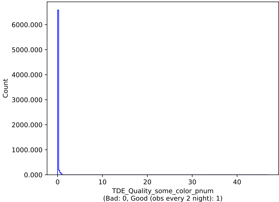
weather_cloudso30v3.4_10yrs : TDE_Quality_some_color_pnum
