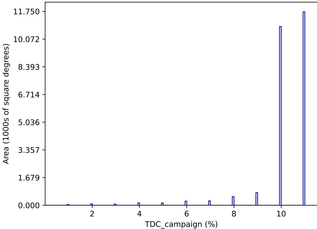
weather_cloudso30v3.4_10yrs : TDC_campaign
