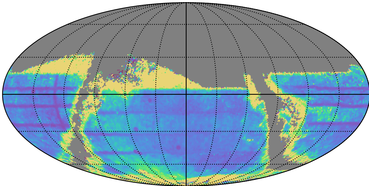
weather_cloudso30v3.4_10yrs : TDC_cadence
