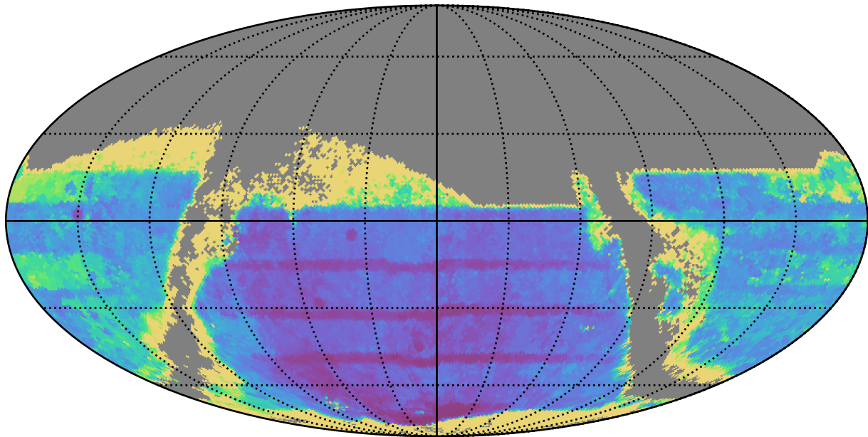
weather_cloudso30v3.4_10yrs : TDC_accuracy
