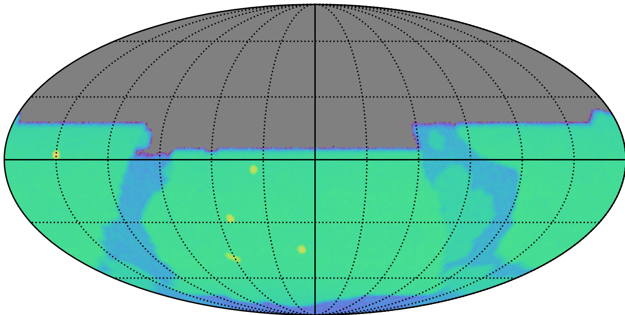
weather_cloudso30v3.4_10yrs y: SurfaceBrightLimit
