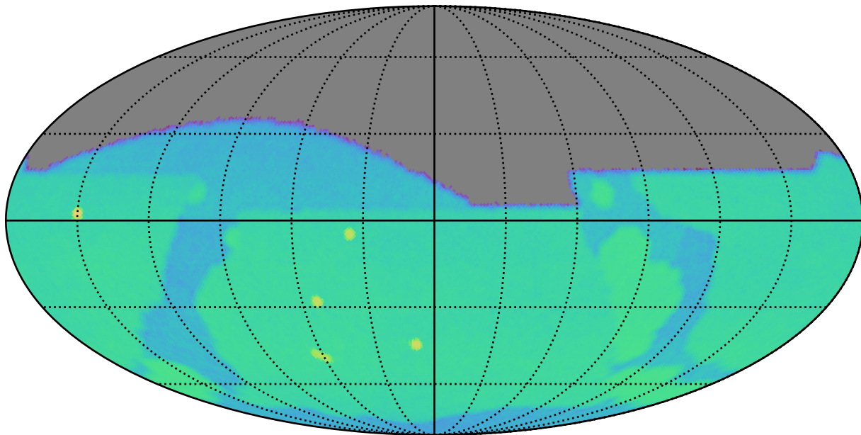
weather_cloudso30v3.4_10yrs g: SurfaceBrightLimit
