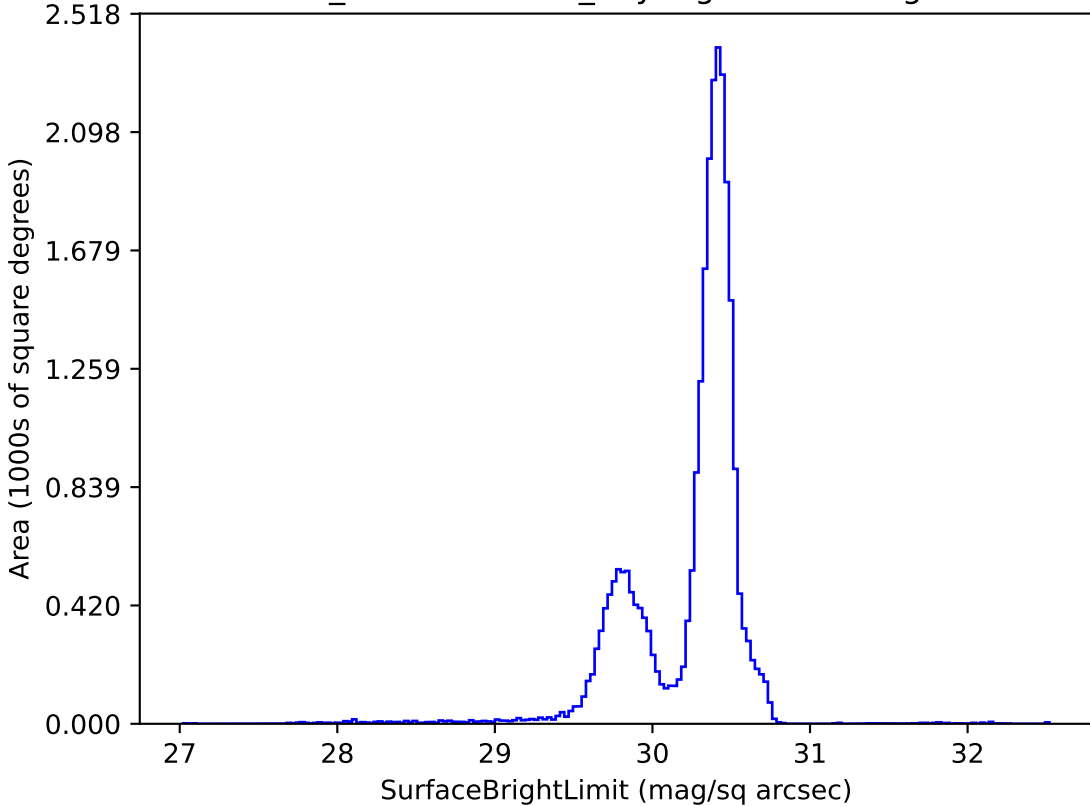
weather_cloudso30v3.4_10yrs g: SurfaceBrightLimit
