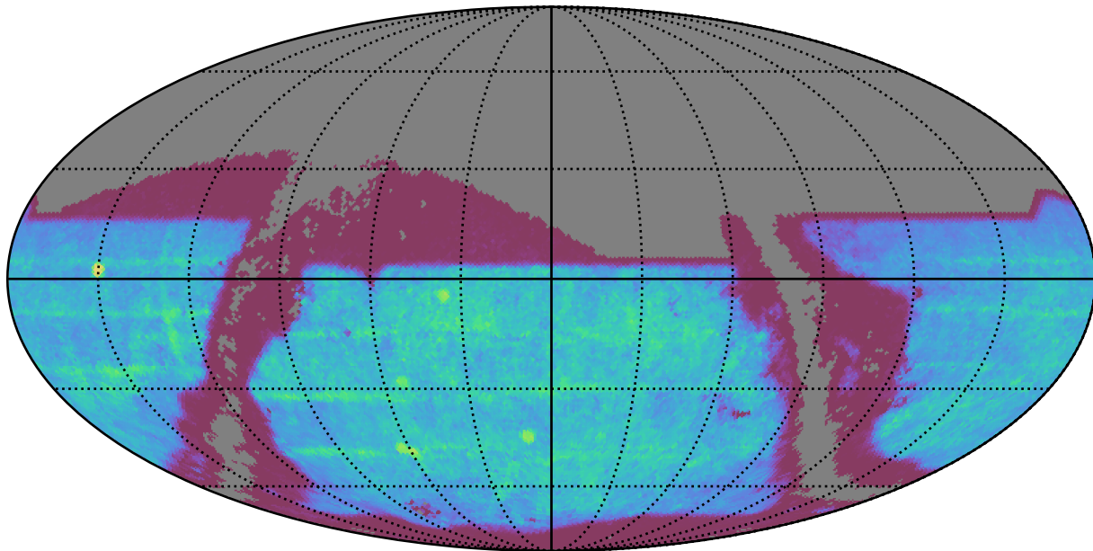
weather_cloudso30v3.4_10yrs : SNSLMetric
