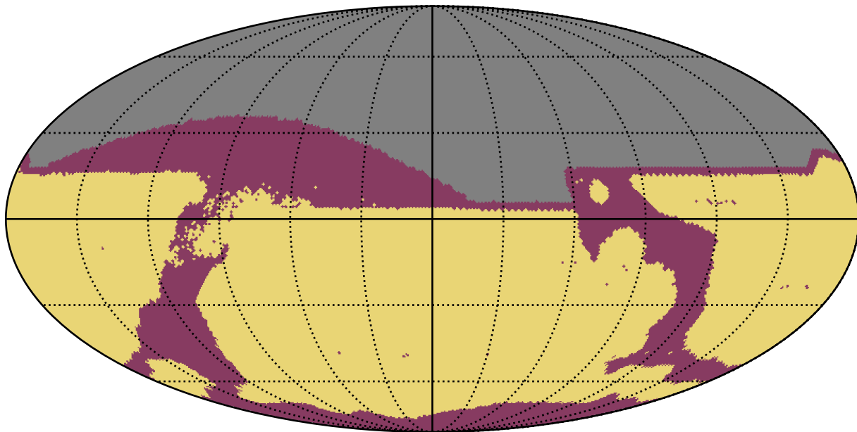
weather_cloudso30v3.4_10yrs : RapidRevisits
