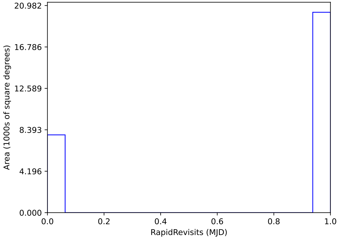
weather_cloudso30v3.4_10yrs : RapidRevisits
