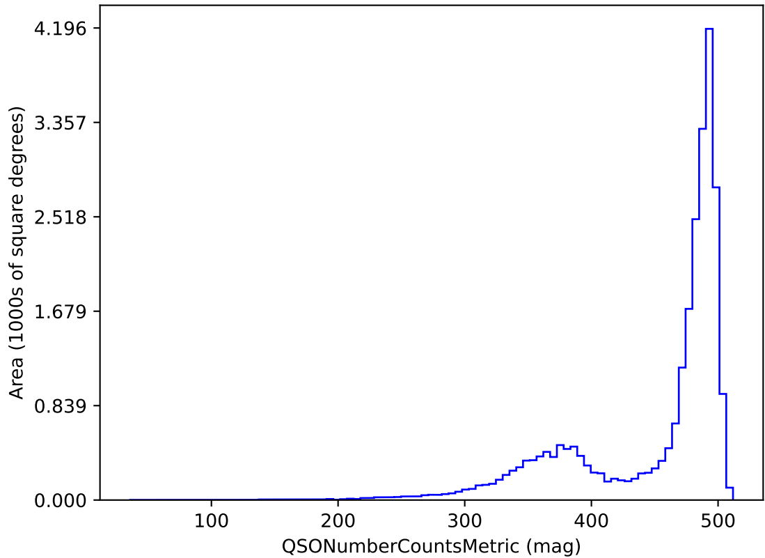
weather_cloudso30v3.4_10yrs z band and non-DD: QSONumberCountsMetric
