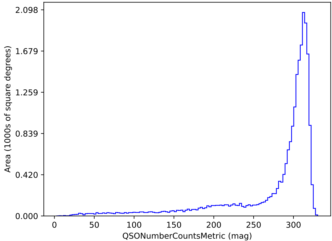
weather_cloudso30v3.4_10yrs u band and non-DD: QSONumberCountsMetric
