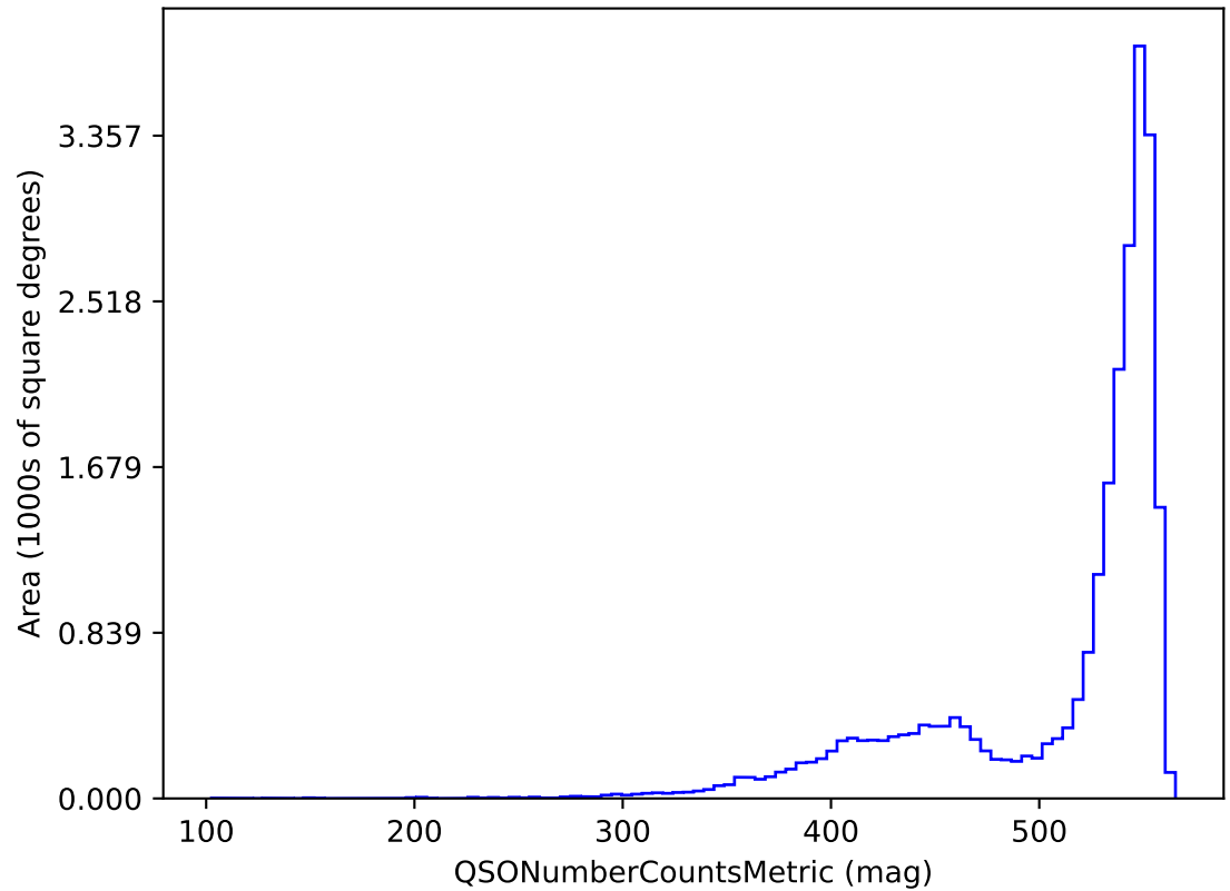
weather_cloudso30v3.4_10yrs i band and non-DD: QSONumberCountsMetric
