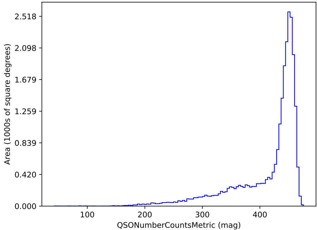
weather_cloudso30v3.4_10yrs g band and non-DD: QSONumberCountsMetric
