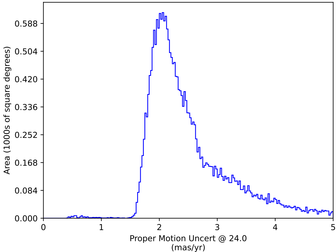
weather_cloudso30v3.4_10yrs : Proper Motion Uncert @ 24.0
