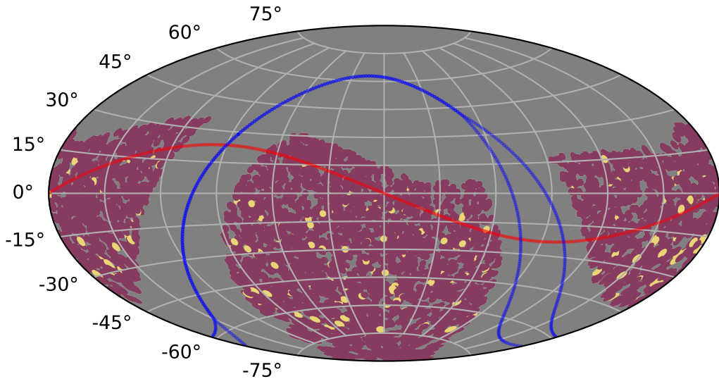
weather_cloudso30v3.4_10yrs : PrestoKNe_score_s
