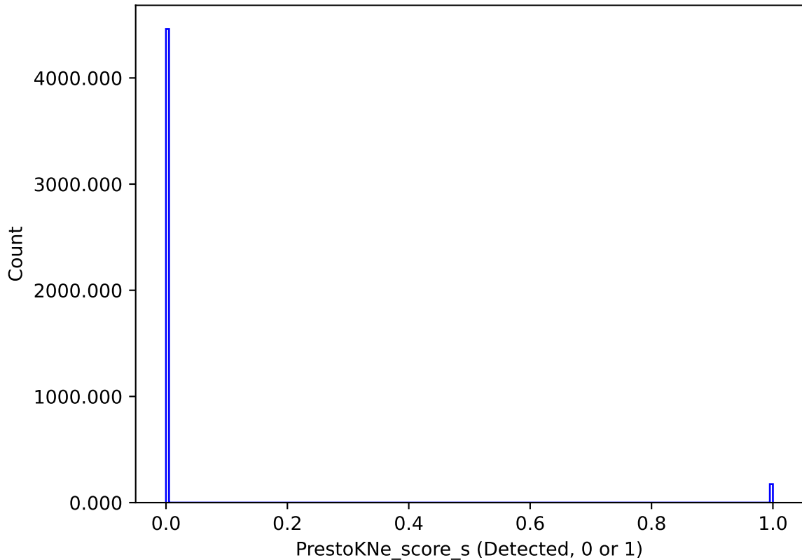
weather_cloudso30v3.4_10yrs : PrestoKNe_score_s
