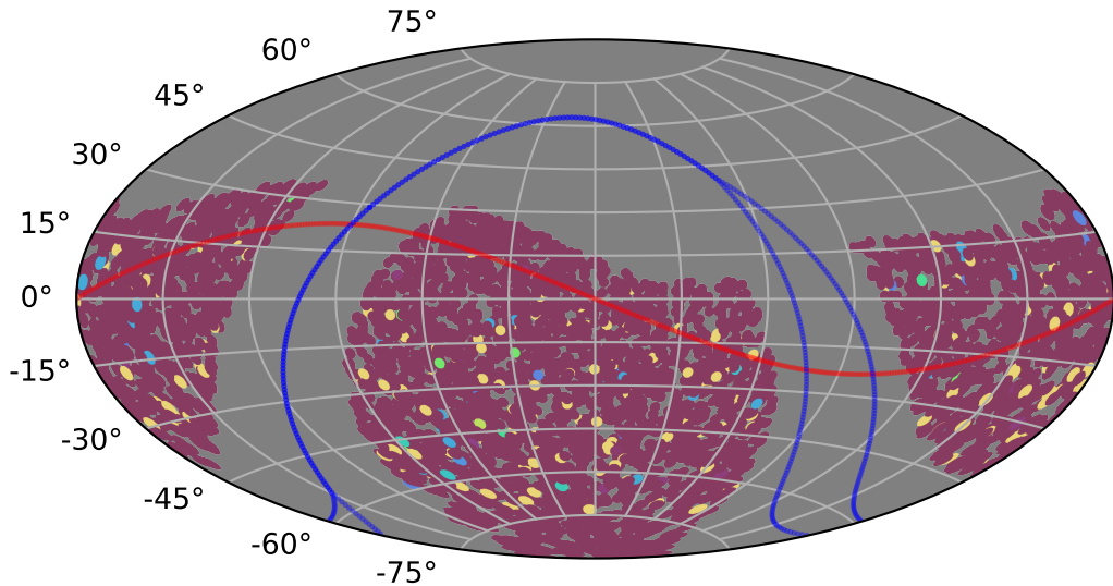
weather_cloudso30v3.4_10yrs : PrestoKNe_score_p
