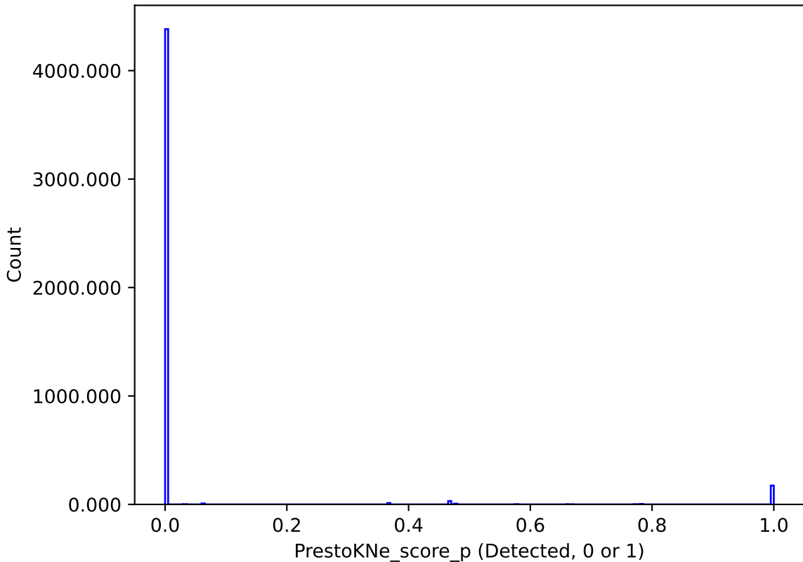
weather_cloudso30v3.4_10yrs : PrestoKNe_score_p
