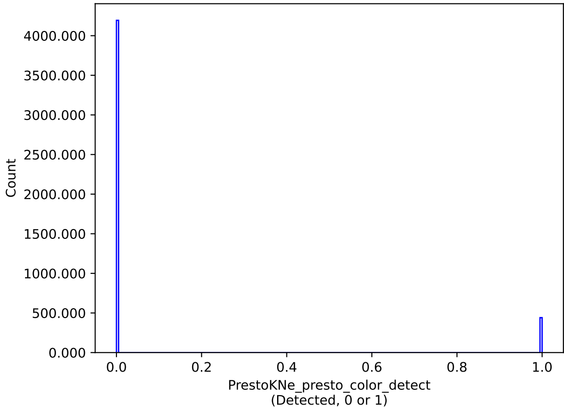
weather_cloudso30v3.4_10yrs : PrestoKNe_presto_color_detect
