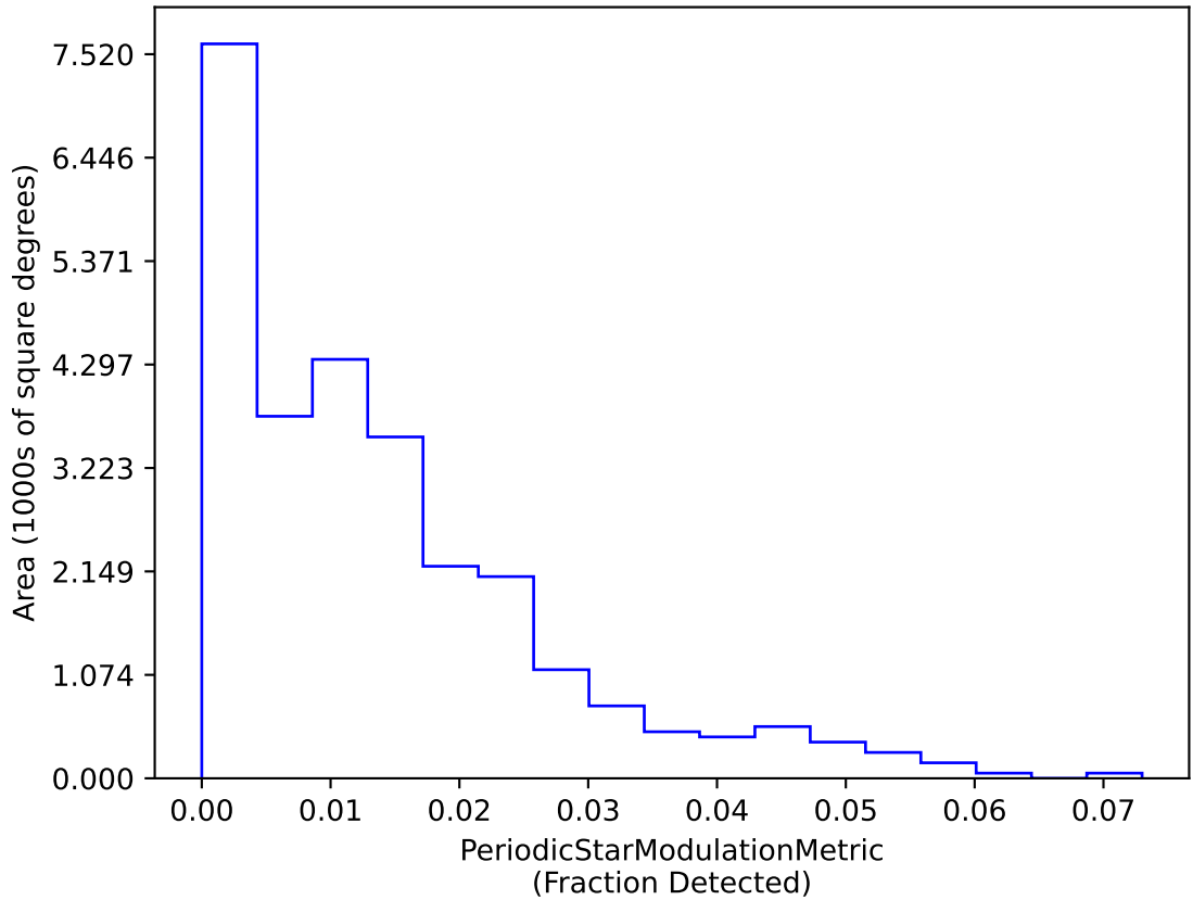
weather_cloudso30v3.4_10yrs dm 21 interval 15 RRC Year 1-2: PeriodicStarModulationMetric
