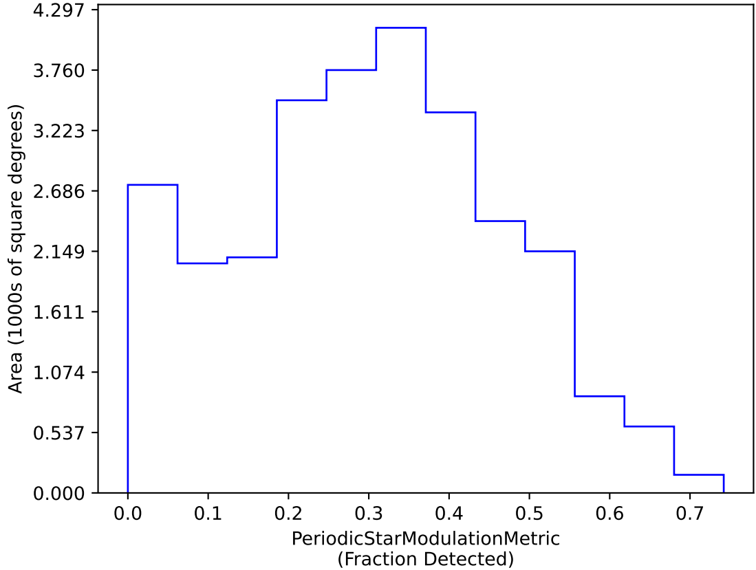
weather_cloudso30v3.4_10yrs dm 19 interval 30 RRC Year 1-2: PeriodicStarModulationMetric
