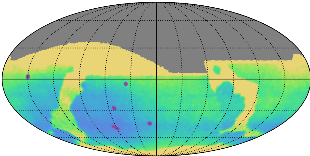
weather_cloudso30v3.4_10yrs : Parallax Uncert @ 24.0
