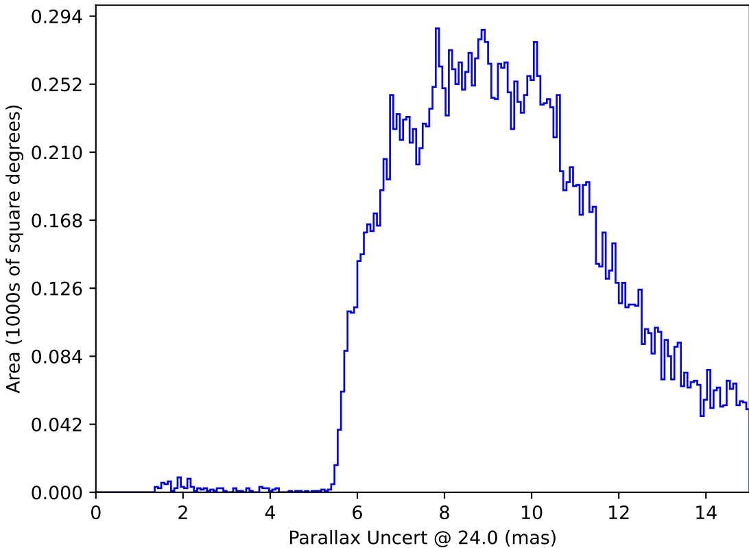
weather_cloudso30v3.4_10yrs : Parallax Uncert @ 24.0
